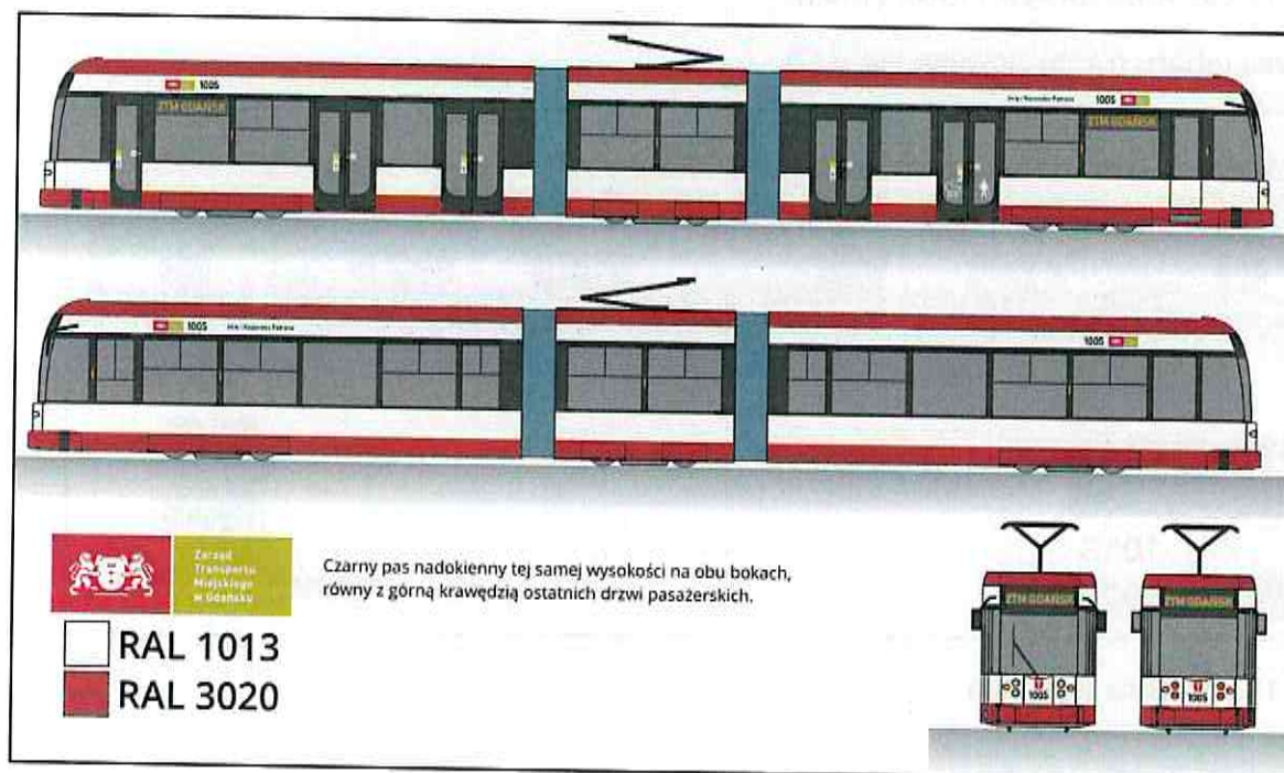
Rys. 12.3.3. Bombardier NGT6
