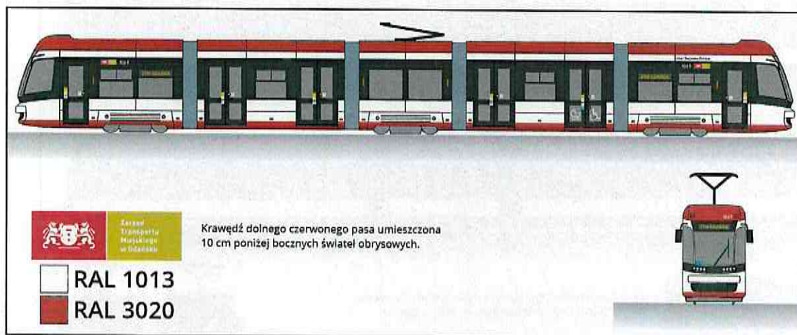
Rys. 12.3.1. Pesa Jazz Duo
