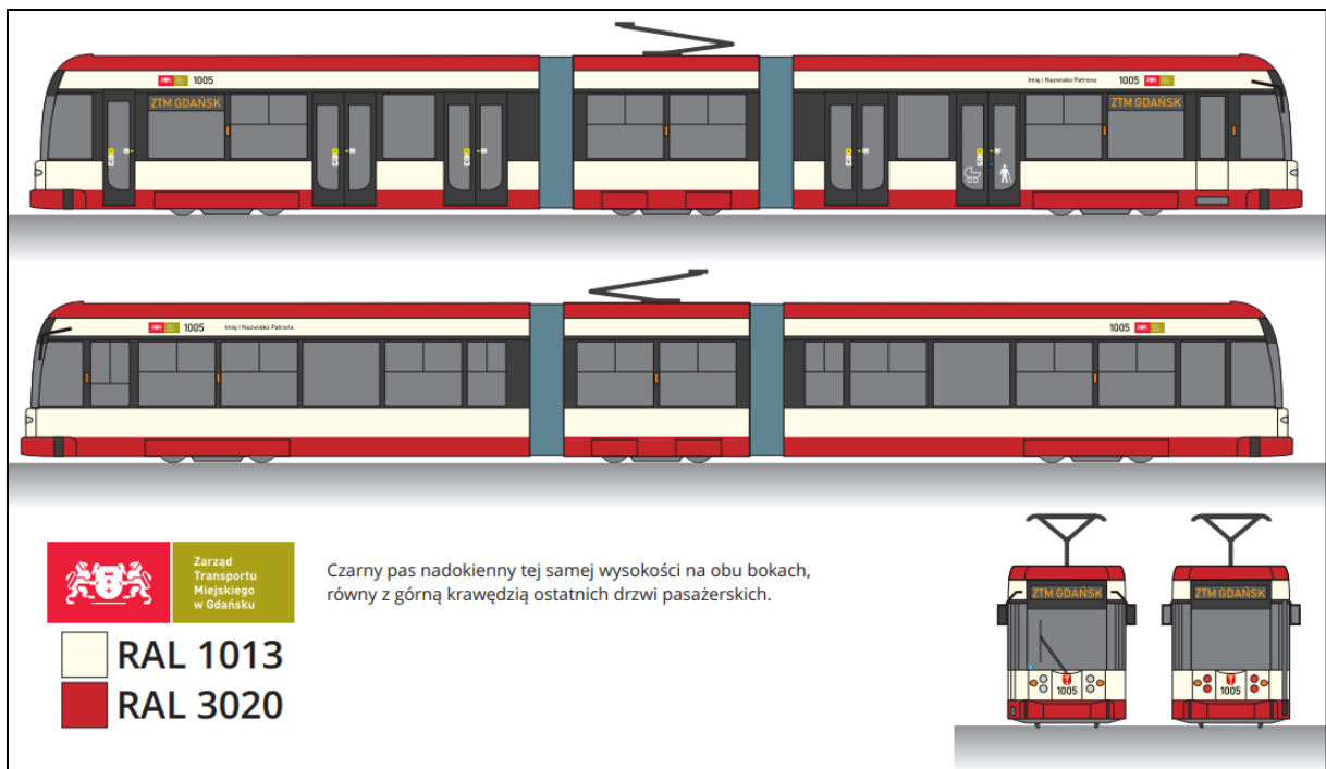
Rys. 12.3.3. Bombardier NGT6
