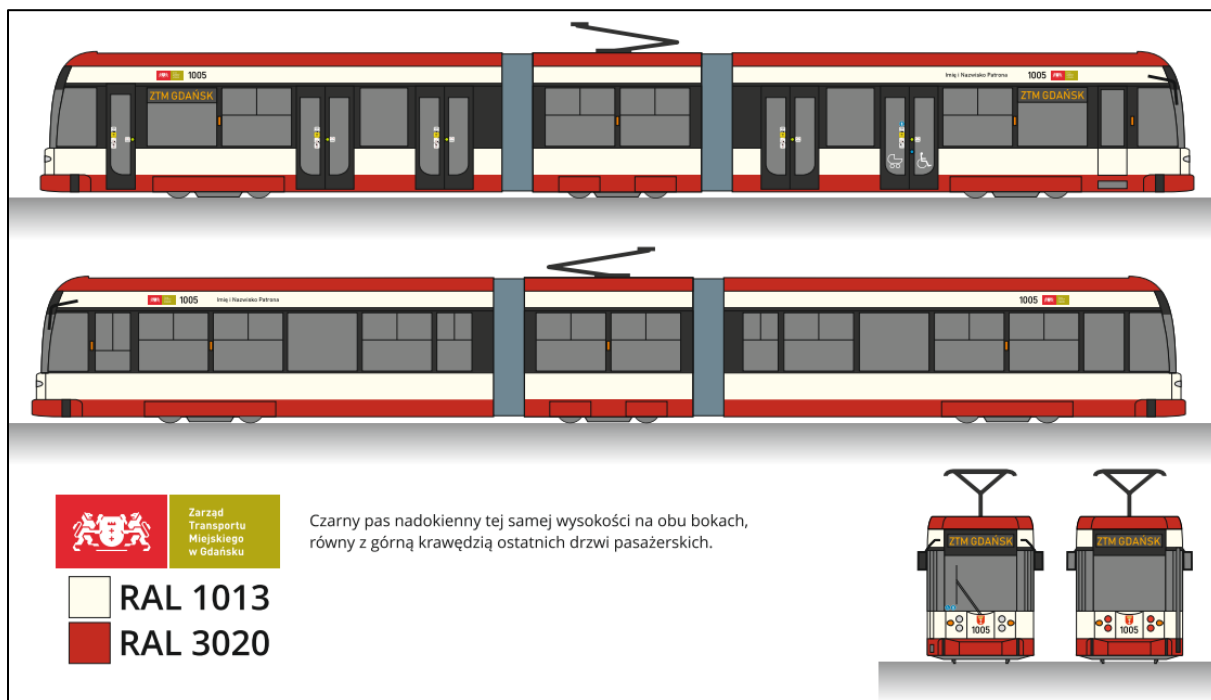
Rys. 12.3.3. Bombardier NGT6
