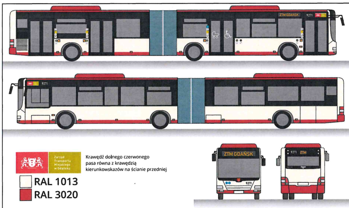
12.7.8. MAN Lion's City G '09
